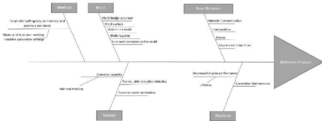
Gambar 3. Diagram Fishbone
